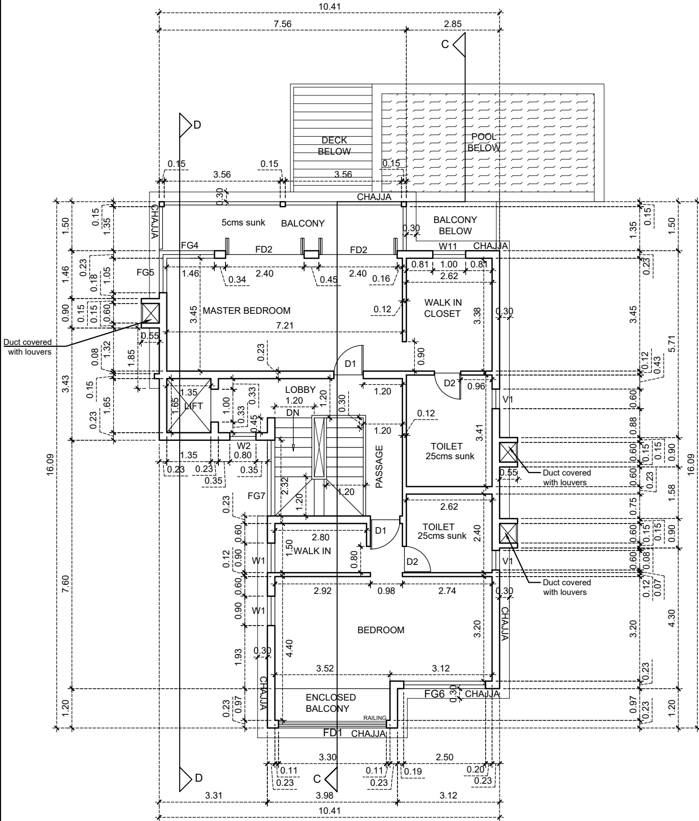
TYPE B - SECOND FLOOR PLAN
